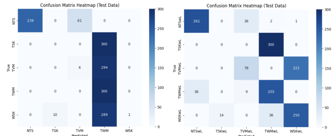
FIGURE 8: The test result for heterogeneous device data using Random Forest
