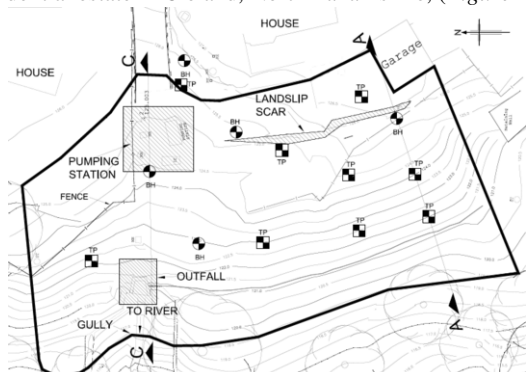
Figure 1. Site plan with marked areas of excessive settlement (shaded regions) and GI locations (BH-borehole, TP-trial pit)
