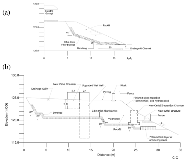
Figure 4. Magnitude of excavation and design of rockfill slope below the landslide scar (a) and around the SPS (b).
