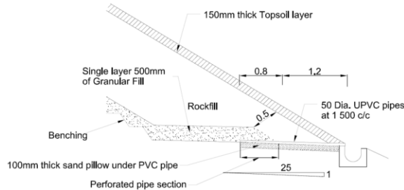
Figure 3. Typical design of filter layer and contour drain channel.
