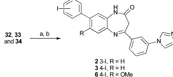
Scheme 5 Reagents and conditions: (a) (\text{Me}_3\text{Sn})_2 , (\text{Ph}_3\text{P})_4\text{Pd} (10 mol%), 1,4-dioxane, 90 °C; (b) NaI, chloramine-T, EtOH, 2 (69%), 3 (42%), 6 (47%).
