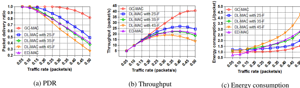
Figure 3: Narrow region scenario: PDR, Throughput, and Energy consumption vs. Traffic rate.
