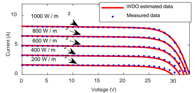
Fig. 7. Comparison of experimental data and WDO estimated data of Kyocera – KC200GT 215 module at different irradiance (double diode model).
