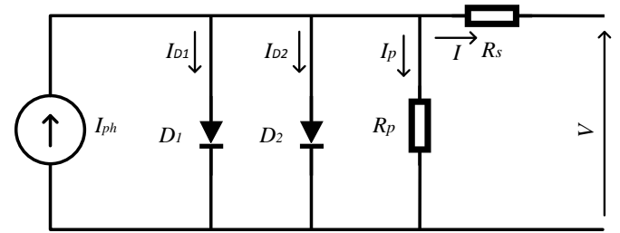
Fig. 2. Double – diode model of solar PV.
