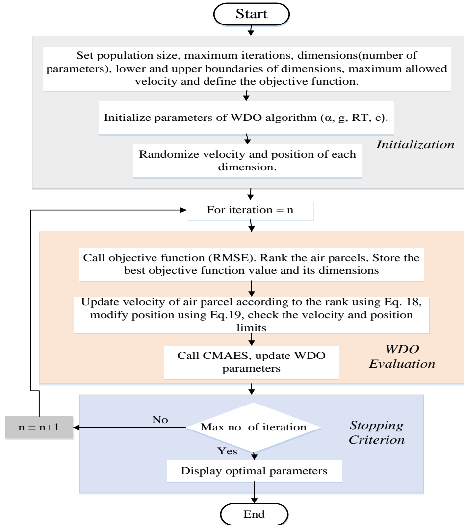
Fig. 3. Flowchart of Wind driven optimization
