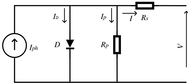
Fig. 1. Single – diode model of solar PV.
