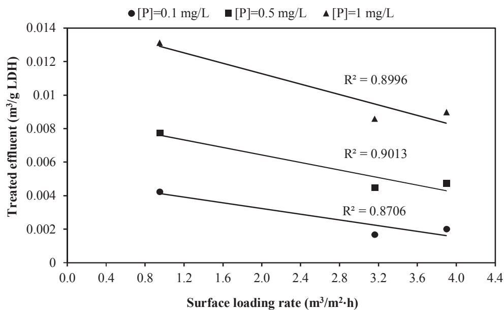
Fig. 3 – Effect of surface loading rate on the treated effluent capacity at different P discharge concentration by Mg-Fe-Cl LDH filled column.
