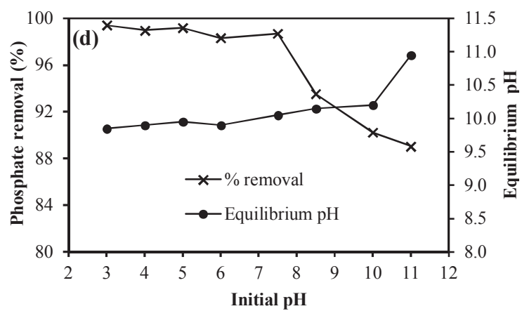
Fig. 1 – Adsorption of phosphate on Mg-Fe-Cl LDH as a function of (a) LDH dosage; (b) contact time; (c) initial phosphate concentration; (d) initial solution pH.
