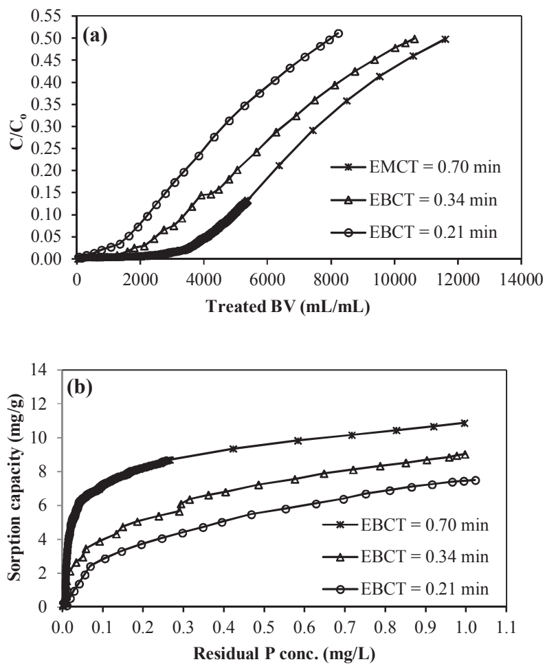
Fig. 2 – Effect of EBCT on phosphate sorption by Mg-Fe-Cl LDH in fixed bed column test: (a) breakthrough curves; (b) sorption capacity.
