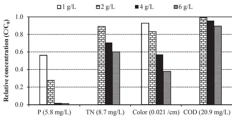
Fig. 4 – Relative residual concentration of various effluent quality parameters after treated by Mg-Fe-Cl-LDH (initial concentrations in parenthesis).
