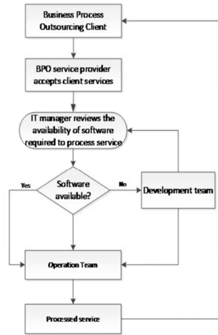
Figure 2. DevOps flowchart.
