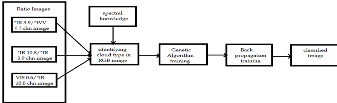
Figure 2-14: The proposed hybrid training method for MLP [23].
