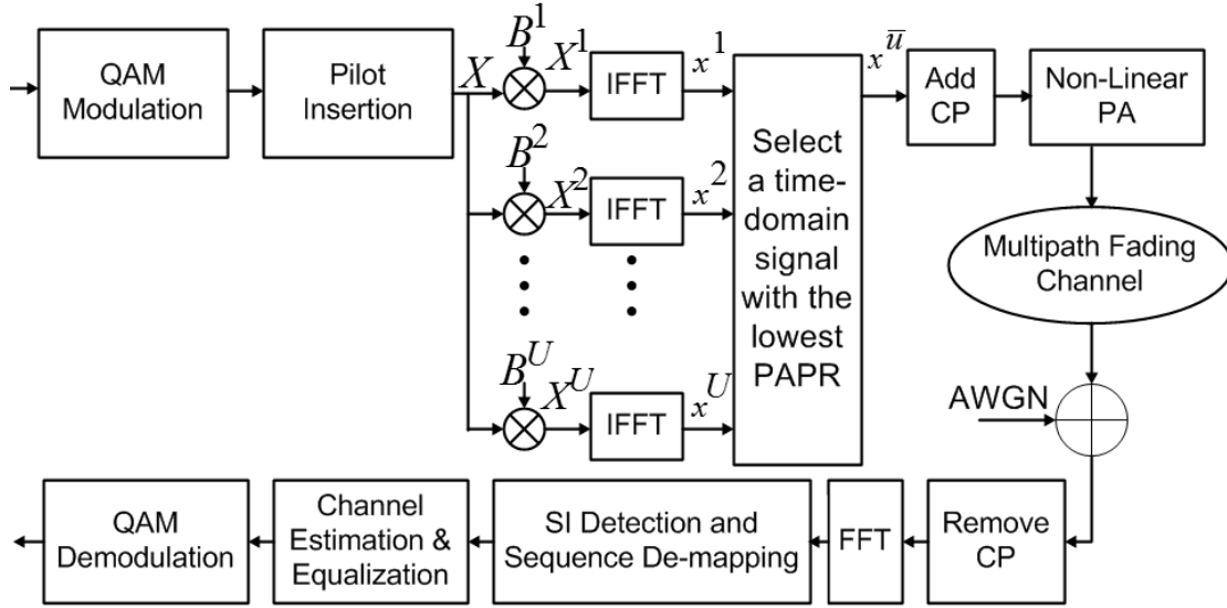
Fig. 1: SLM in pilot-aided OFDM i.e. SLM-OFDM
