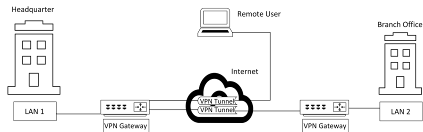
Figure 1. Site-to-site and remote access VPN deployment scenarios.
