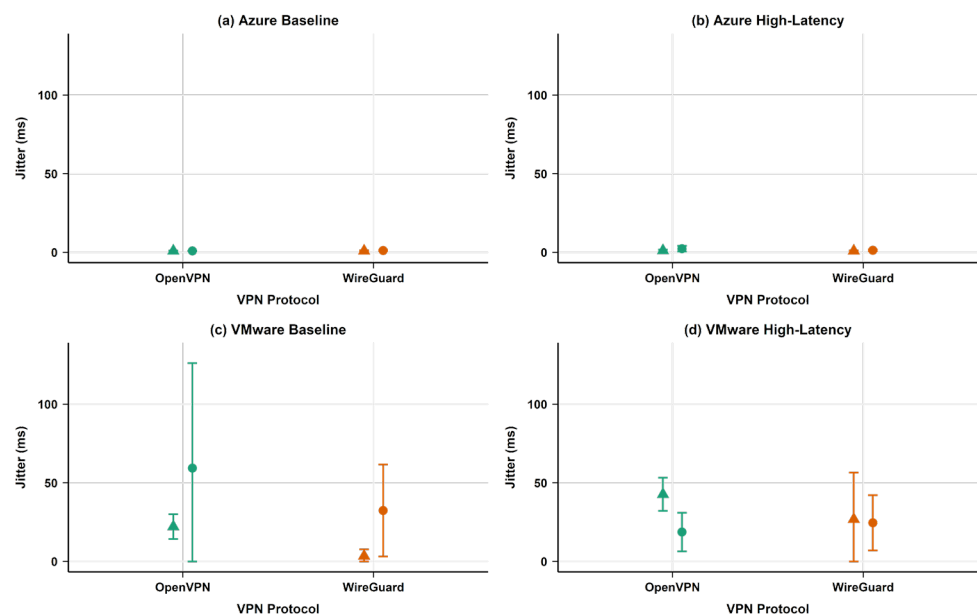
Figure 10. Jitter analysis highlighting VMware's timing variability and WireGuard's superior stability. (Green = OpenVPN, Orange = WireGuard; Triangles = No VPN, Circles = VPN enabled; error bars = 95% CI).
