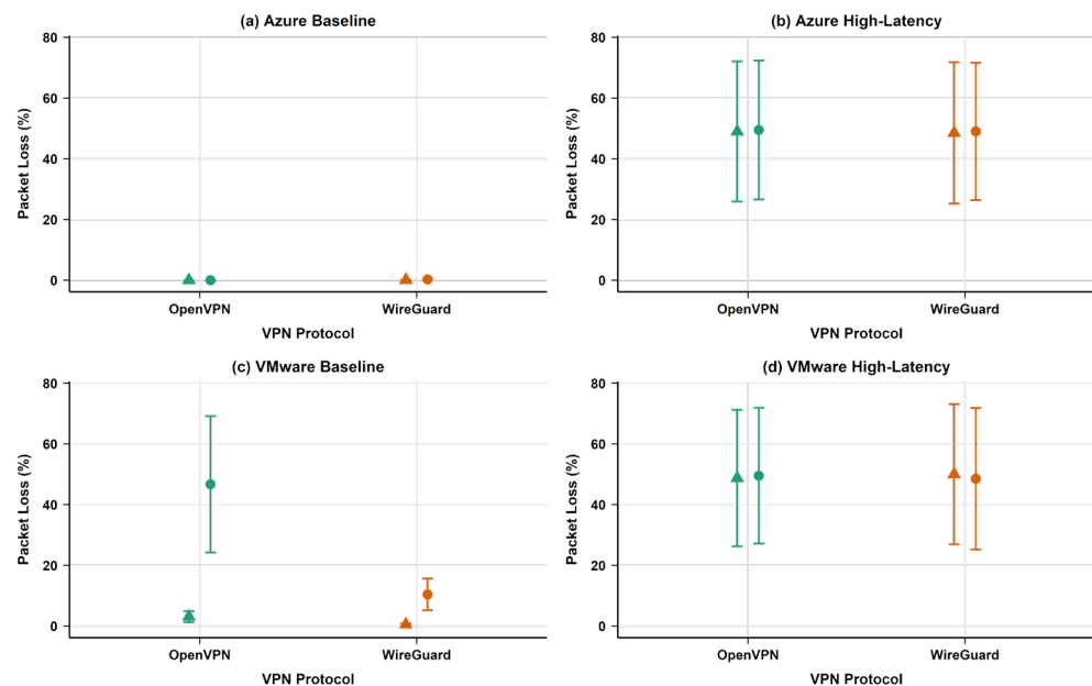
Figure 11. Packet loss rates demonstrating WireGuard’s significant VMware advantage 12.35% vs. 47.01%). (Green = OpenVPN, Orange = WireGuard; Triangles = No VPN, Circles = VPN enabled; error bars = 95% CI).
