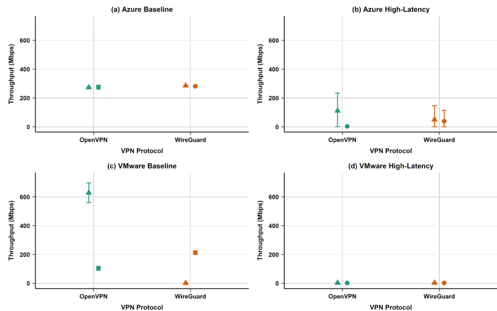
Figure 5. TCP throughput performance across Azure and VMware environments under baseline and high-latency conditions. (Green = OpenVPN, Orange = WireGuard; Triangles = No VPN, Circles = VPN enabled; error bars = 95% CI).
