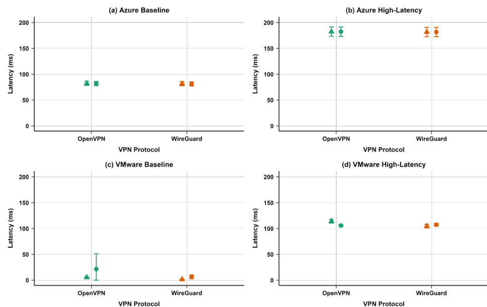
Figure 9. Latency measurements showing minimal protocol differences within environments. (Green = OpenVPN, Orange = WireGuard; Triangles = No VPN, Circles = VPN enabled; error bars = 95% CI).
