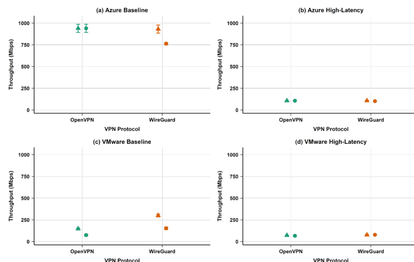
Figure 6. UDP throughput comparison showing environmental dependencies between cloud and virtualised deployments. (Green = OpenVPN, Orange = WireGuard; Triangles = No VPN, Circles = VPN enabled; error bars = 95% CI).
