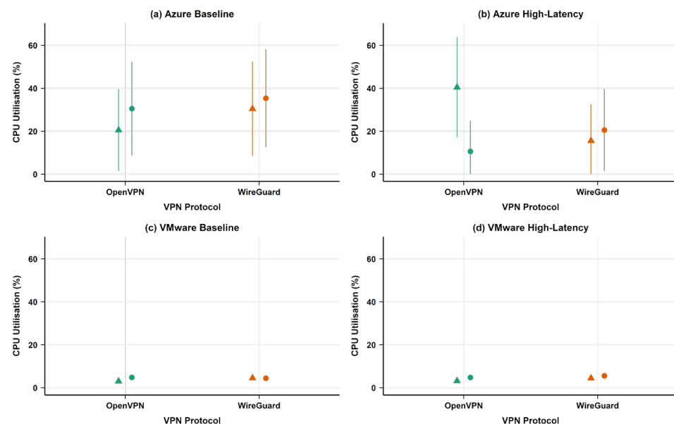
Figure 7. CPU utilisation patterns demonstrating greater environmental than protocol influence. (Green = OpenVPN, Orange = WireGuard; Triangles = No VPN, Circles = VPN enabled; error bars = 95% CI).
