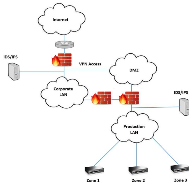
Fig. 2. DMZ with separation of trust zones.
